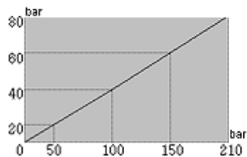
HYDRAURIC PRESS
